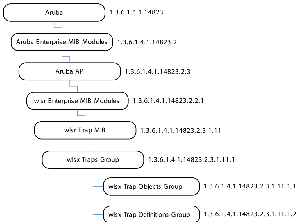
Figure 16 Trap Hierarchy
